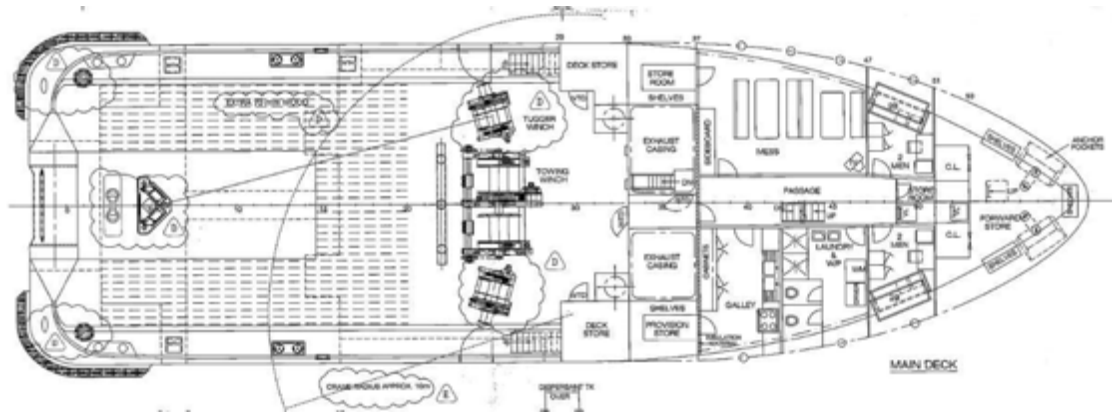
MAIN DECK VIEW
