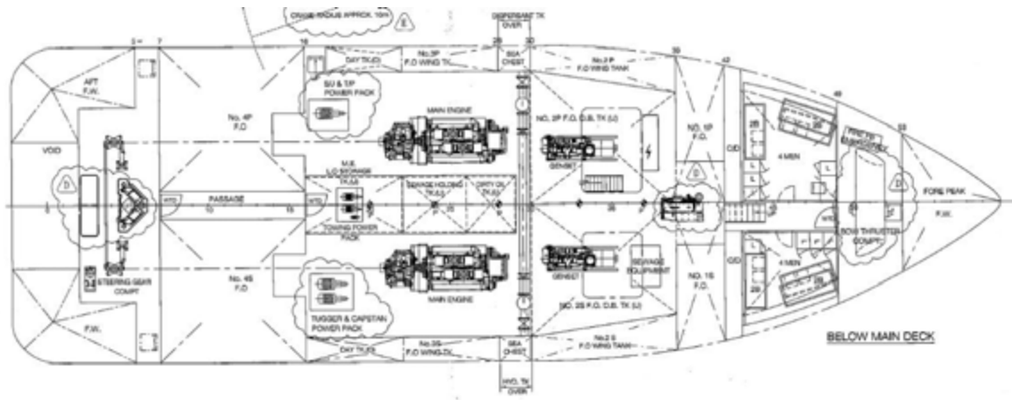
BELOW MAIN DECK VIEW
